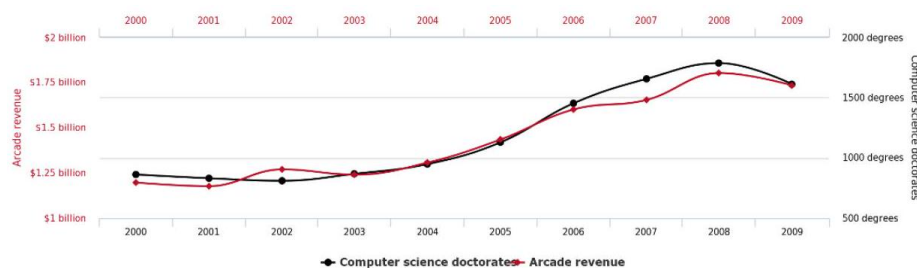
Figure 7.10: the number of Computer Science Ph.Ds awarded each year in the United States strongly correlates with video/pinball arcade revenue. (from Vig15)
